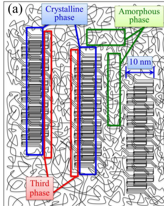
Figure 2-1 - Representation of the three major phases of UHMWPE: Crystalline phase, amorphous phase, and the third interphase. (Permission from Pezzotti G. Raman spectroscopy of biomedical polyethylenes. Acta Biomater. 2017 Jun 1;55:28–99. DOI: 10.1016/j.actbio.2017.03.015)
