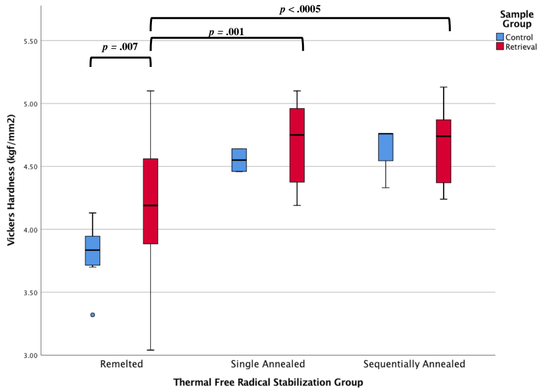
Figure 5-4 - Comparison of hardness values for control and retrieved liner rims grouped according to their thermal stabilization. Note that statistically significant differences were found in Vickers hardness between retrieved remelted liner rims compared to both single and sequentially annealed liner rims, as well as between remelted control and retrieved liner rims.
